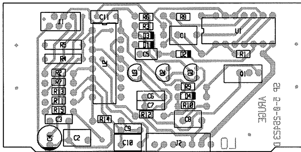
View from component side with lower side tracks. PCB rev. 26423D
