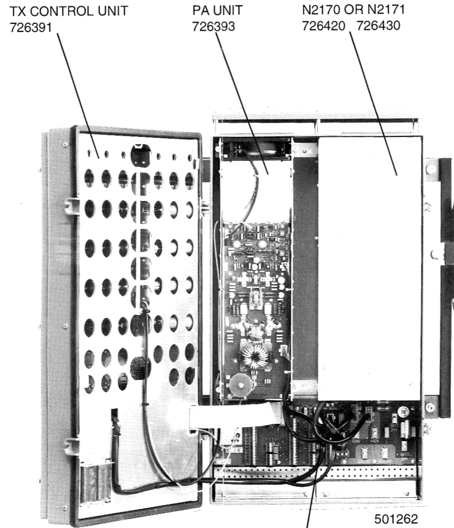
CONNECTION BOARD (13) 626413
