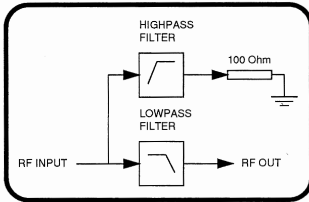
FILTER 1 TO 6
