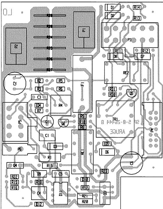
View from component side with lower side tracks. PCB rev. 26444B
